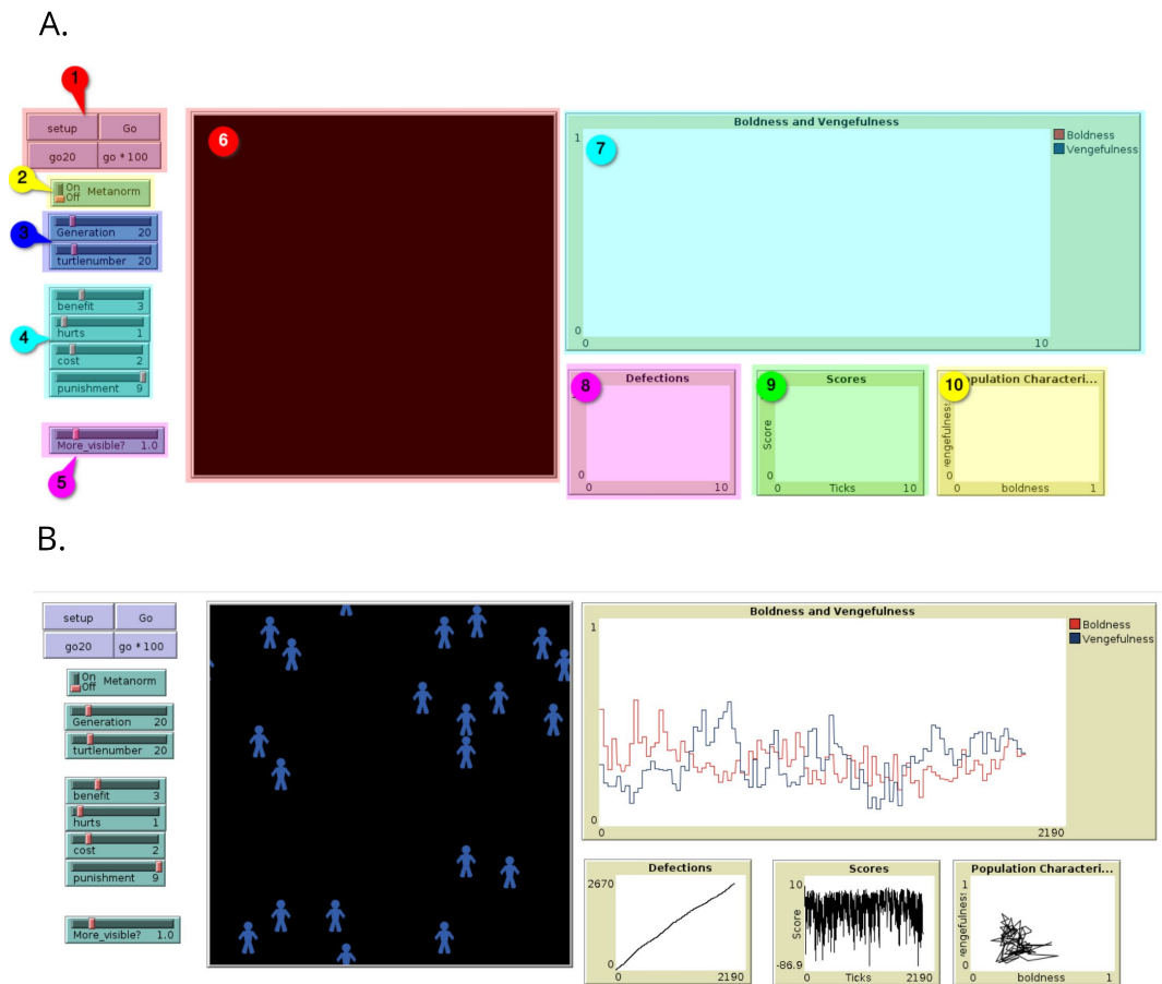
Figure 3. Screenshot of the NetLogo implementation of the Norms and Metanorms game. In A, the NetLogo interface with the elements that control the simulation runs: 1. Control buttons to set up and run the simulation; 2. Switcher to turn Metanorms game on or off; 3. Slider to define the number of agents and the number of agents decisions which conform a generation; 5. Slider to define the value of the seen? variable; 6. World in which the environment and agents are instantiated; 7. Chart of the evolution of boldness and vengefulness variables across the generations; 8. Chart of the number of defections by generation; 9. Chart of scores by generation; and 10. Scatter plot of boldness versus vengefulness across generations. In B, the NetLogo Interface after 100 generations of the Norms game.
