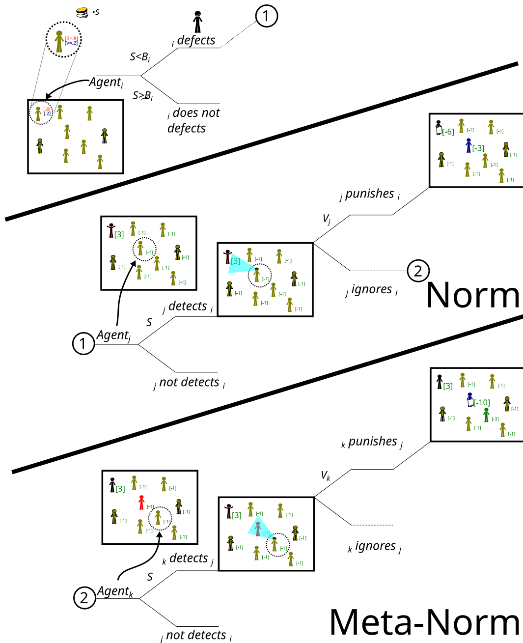
Figure 2. Algorithm structure of the Norms and Metanorms game. S represents the global variable seen? , letters i, j and k represent different agent sets and roles. Person-like shapes graphically represent agents and adjacent numbers represent their scores.
